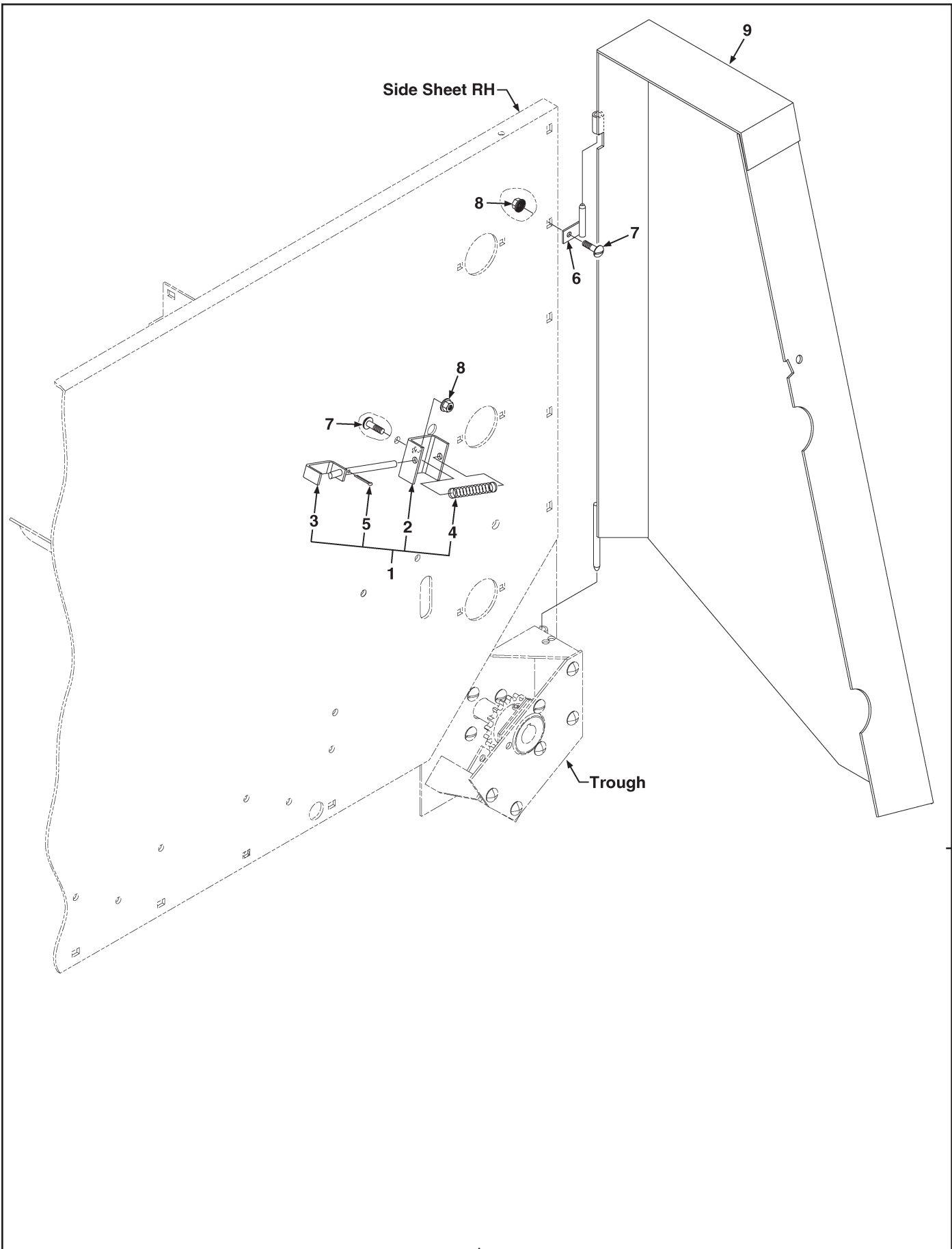
Figure 9. Shield Assembly & Related Parts
