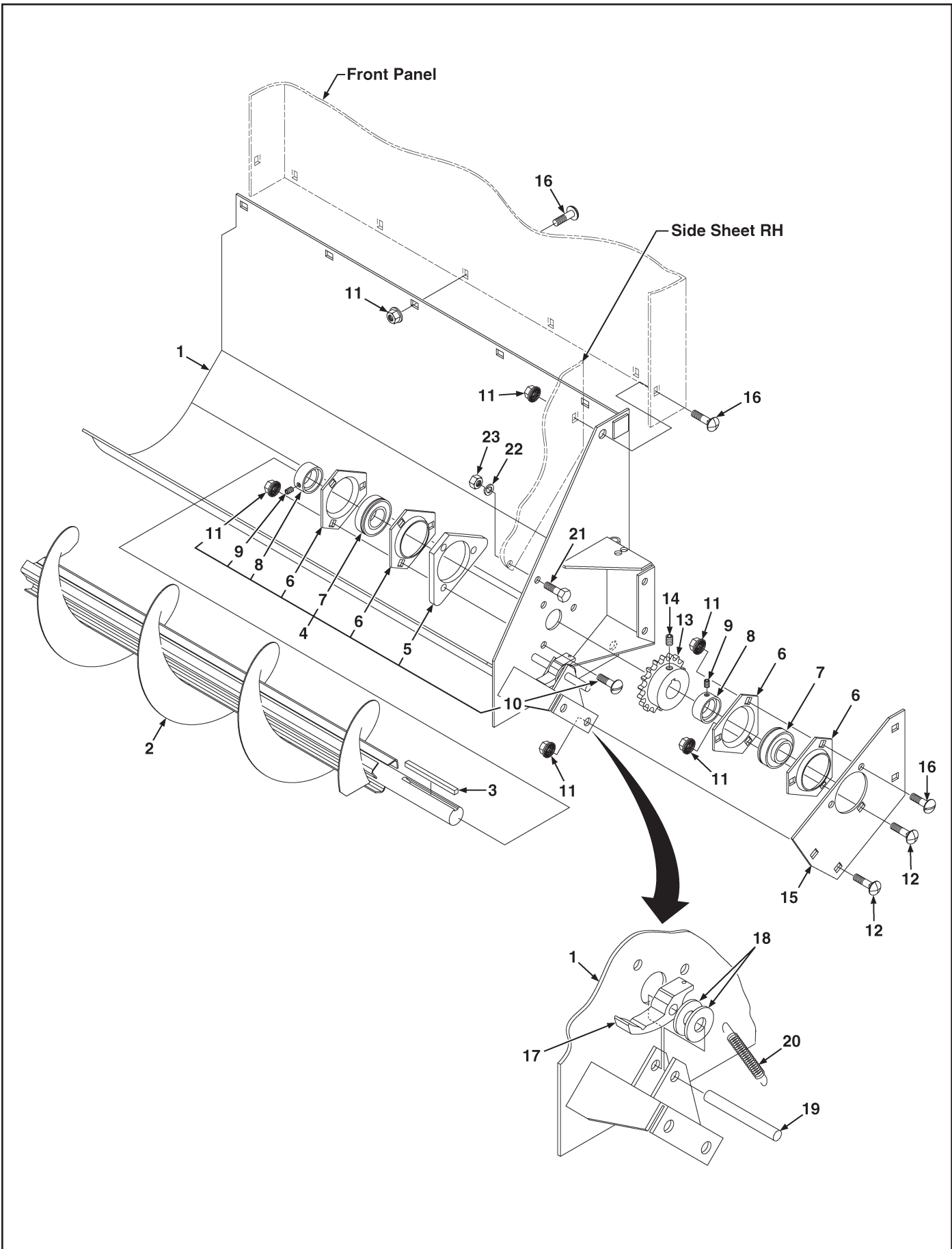
Figure 3. Trough, Auger & Related Parts
